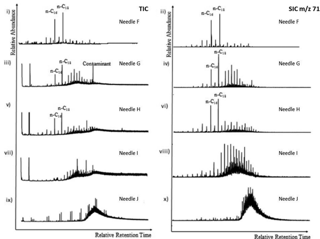
Fig. 6 Total ion chromatogram (TIC) and single ion chromatogram (SIC) m/z 71 of volatiles released from needles F–H in HyPy and needles I–J in NPy. n\text{-C}_{16} = hexadecane; n\text{-C}_{18} = octadecane.
